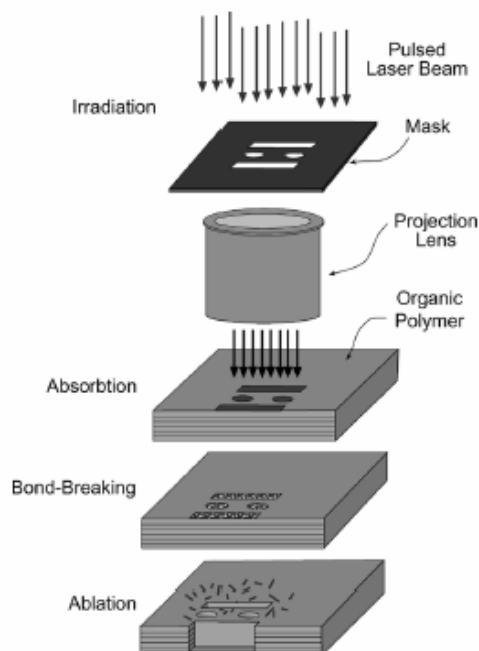
Figure 5 – Schematic of the laser ablation process [10].
