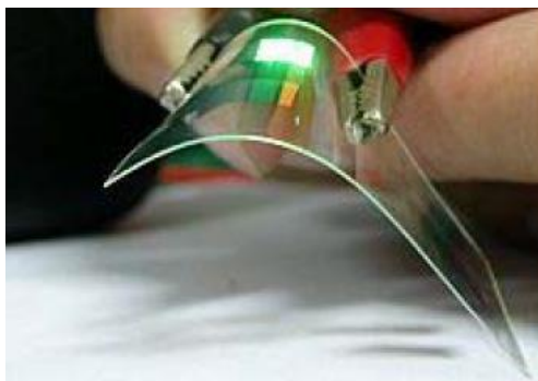
Figure 14 - Demonstration of a flexible OLED device. Photo: General Electric
